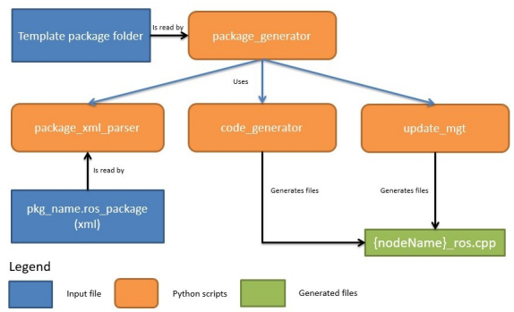
Figure 2: Main components of the package generator.
